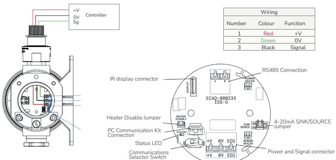
Figure 7: Sink/source jumper location
