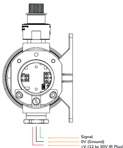
Figure 3: Field cable connections on the IR Plus
